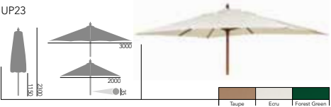
Rectangular Parasol w/ Pulley 2.0m x 3.0m
