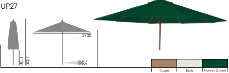
Round Parasol w/ Pulley 2.7mØ
